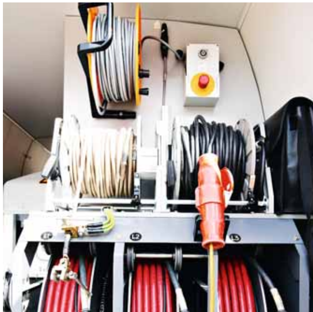
Kabelmesswagen
